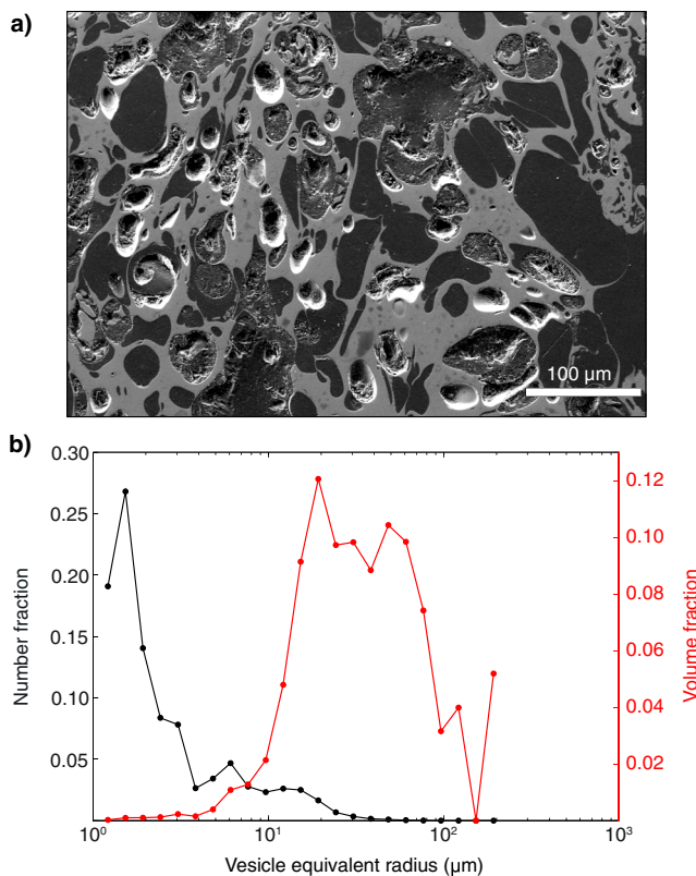
Figure 4. (a) Backscattered scanning electron microscope image of a typical fallout Plinian pumice from the Glass Mountain eruption. Vesicles appear in dark gray and the glass in light gray. (b) Vesicle number (black) and volume (red) fractions obtained by image analysis. Number density is dominated by vesicles with a radius < 5 \mu\text{m} , while volume is dominated by vesicles 20\text{--}50 \mu\text{m} . The average vesicle radius is 12.1 \mu\text{m} .
