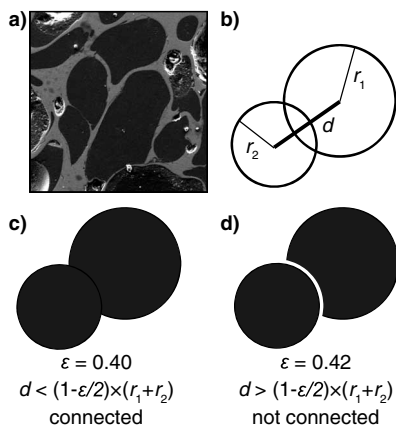
Figure 3. Illustration of the geometrical parameter \epsilon used in the percolation model (Blower, 2001a, 2001b). (a) SEM image of a Glass Mountain pumice showing that vesicles can be nonspherical, representing deformed bubbles that were separated by thin films of melt. (b) Two overlapping spheres of radii r_1 and r_2 . (c) At a value of \epsilon = 0.40 , corresponding to d < (1 - \epsilon/2) \times (r_1 + r_2) , the two spheres are considered connected (coalesced) and gas can flow between them. (d) At a value of \epsilon = 0.42 , corresponding to d > (1 - \epsilon/2) \times (r_1 + r_2) , the two overlapping spheres are considered isolated and gas cannot flow between them.
