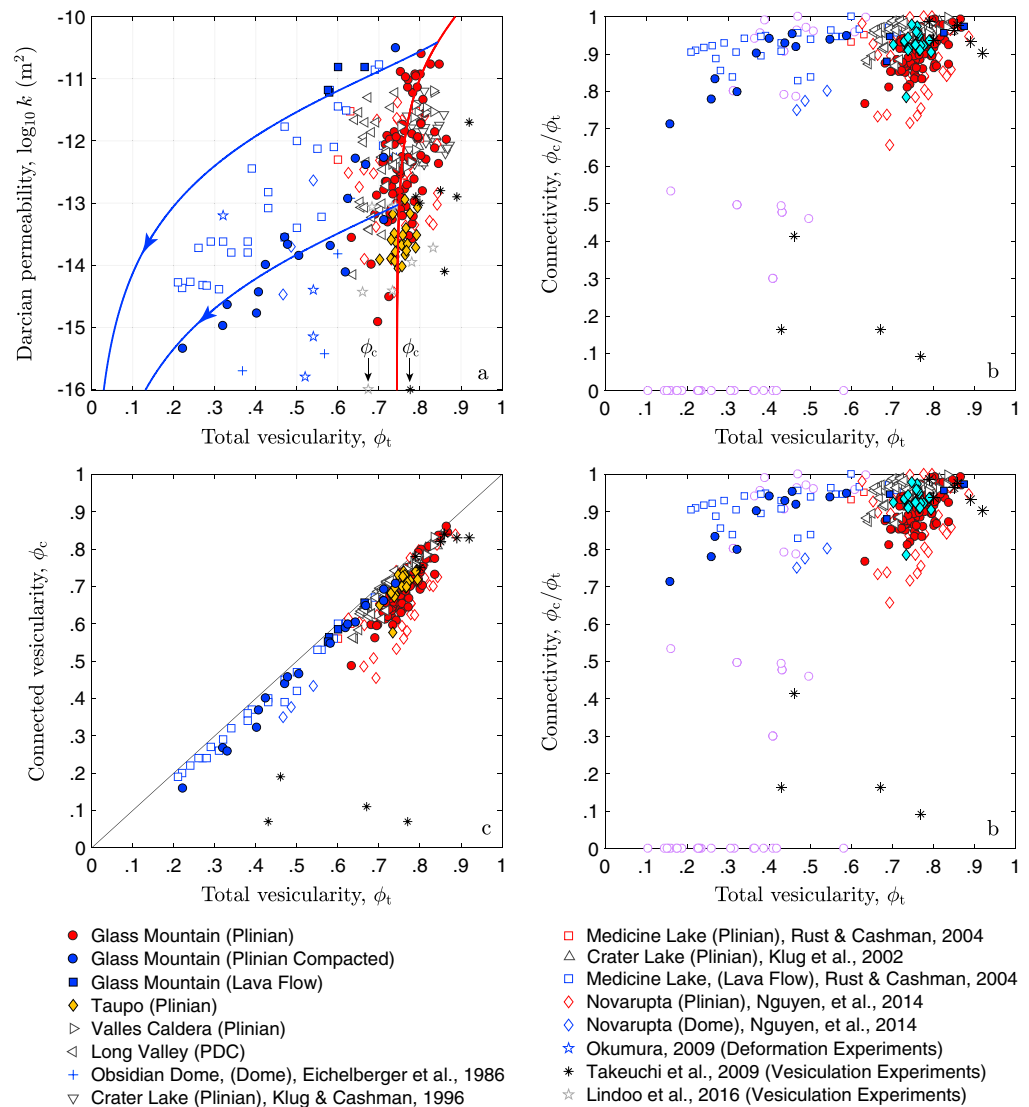
Figure 11. Data from Glass Mountain samples, other explosive and effusive eruptions, and experiments. (a) Log of Darcian permeability, k , as a function of total vesicularity, \phi_t . The red curve represents the fit to Glass Mountain Plinian data (equation (2)) and the blue curves are based on equation (11). The arrows labeled \phi_{cr} indicate the maximum value of \phi_t for which permeabilities were below the detection limit ( \sim 10^{-17} \text{ m}^2 for Takeuchi et al., 2009 and < 10^{-15} \text{ m}^2 for Lindoo, 2016). (b) Connectivity, \phi_c/\phi_t , as a function of total porosity. (c) Connected volume fraction of vesicles, \phi_c , versus total porosity. (d) Log of Darcian permeability as a function of connectivity. Note the outliers in Figures 11b and 11c are for experiments with undetectable permeabilities.
