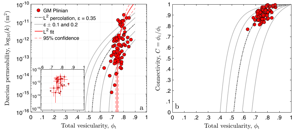
Figure 2. (a) Darcian permeability, k , vs. total porosity, \phi_t , for individual cores taken from the Glass Mountain pumice clasts (Plinian fall). Measurement limit on k is approximately 10^{-17} \text{ m}^2 . The red curve represents the least squares fit to the measured values of \phi_t as a function of k , based on equation (2), with dashed red curves showing the 95% confidence interval. Inset shows the range in values obtained from multiple cores of the same clast with the mean value of \log_{10}(k) and \phi_t shown as filled circles and the vertical and horizontal bars indicating the range in values for the given clast. (b) Corresponding connectivity, C , versus total porosity, \phi_t . The solid gray curve is the least squares fit to \phi_c as a function of \phi_t obtained from percolation modeling with \epsilon = 0.35 , corresponding to estimated values of \phi_{cr} = 0.52 , b = 0.42 , and n = 2.87 . Also shown as gray dashed curves are results from percolation modeling for \epsilon = 0.15, 0.25, 0.45, 0.55 , corresponding respectively to \phi_{cr} = 0.40, 0.45, 0.59 , and 0.66 , as well as b = 1.04, 0.69, 0.22, 0.13 , and n = 3.21, 3.07, 2.66, 2.49 .
